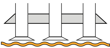
PLACING RACKS NEAR OR ON THE JOINT
