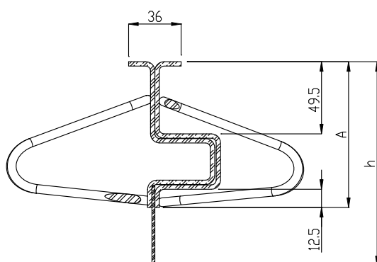
cross section
